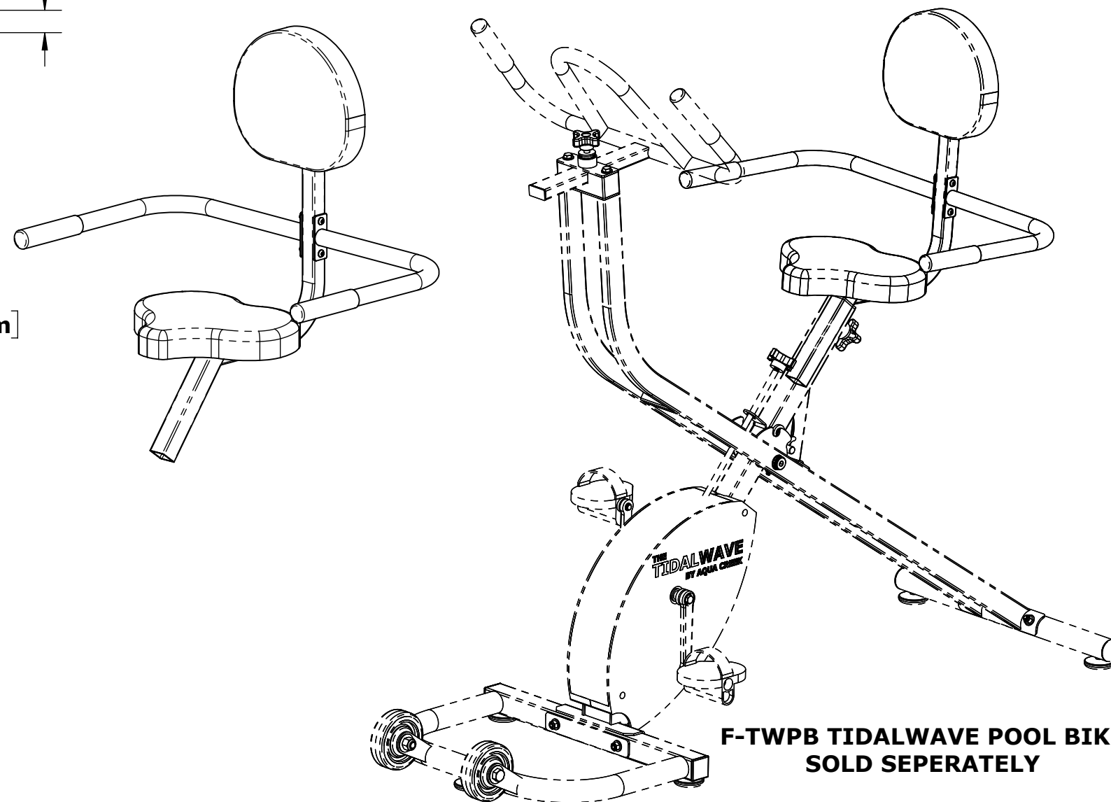
SEAT ADJUSTMENT
