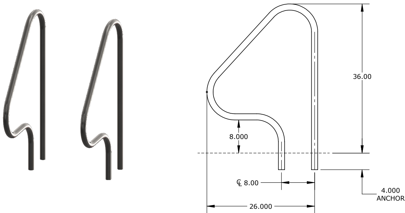
FIGURE 4 GRAB RAIL - 26.00" SETBACK - 1.50" OD X .120 WALL - 316LSS
