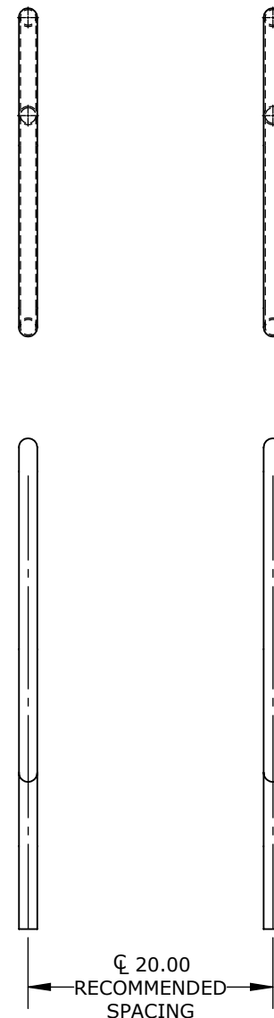
FIGURE 4 GRAB RAIL - 26.00" SETBACK - 1.50" OD X .120 WALL - 316LSS
