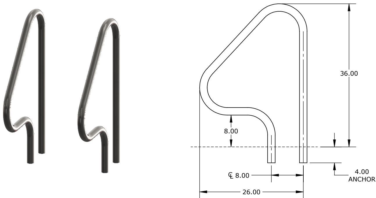
FIGURE 4 GRAB RAIL - 26.00" SETBACK - 1.90" OD X .065 WALL - 304LSS
