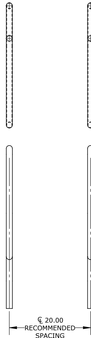
FIGURE 4 GRAB RAIL - 30.00" SETBACK - 1.50" OD X .120 WALL - 316LSS
