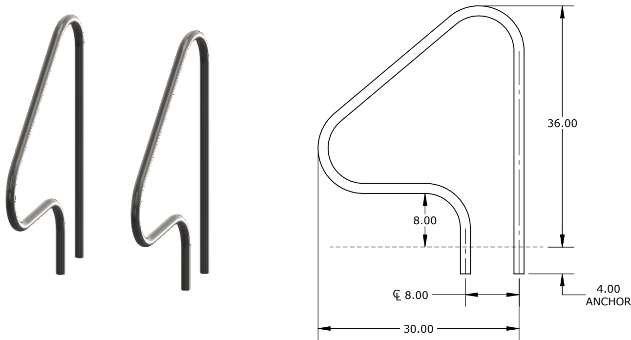
FIGURE 4 GRAB RAIL - 30.00" SETBACK - 1.50" OD X .120 WALL - 316LSS
