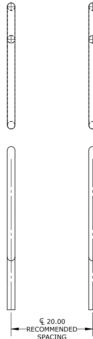
FIGURE 4 GRAB RAIL - 30.00" SETBACK - 1.90" OD X .065 WALL - 304LSS
