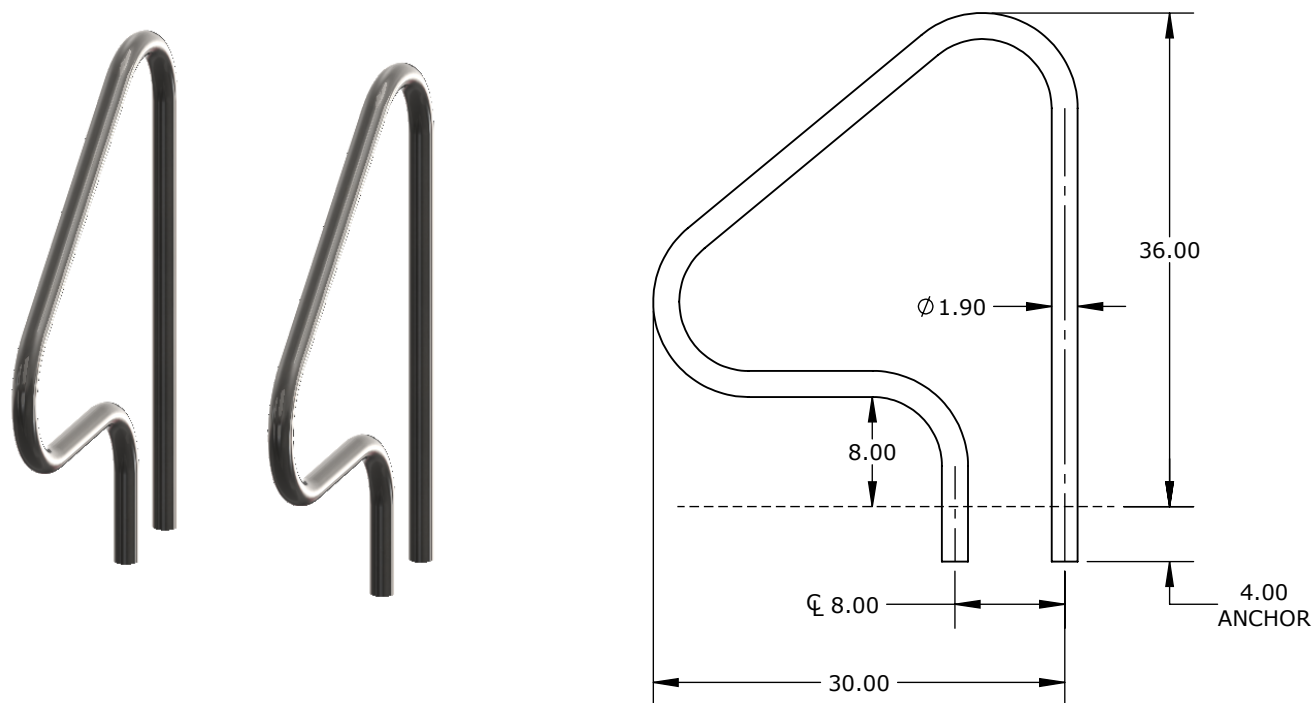
FIGURE 4 GRAB RAIL - 30.00" SETBACK - 1.90" OD X .065 WALL - 304LSS
